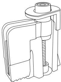
Figure 2 Dog Leg Bracket ready to be installed.
