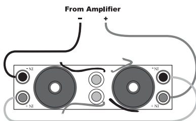
Figure 5 Series Wiring Connections
