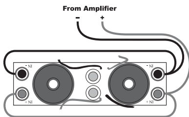
Figure 4 Parallel Wiring Connections
