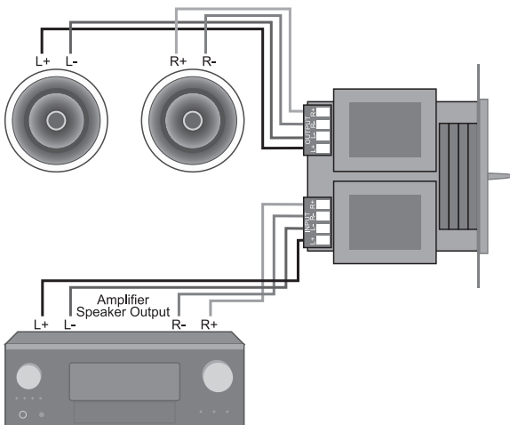
Wiring Diagram
